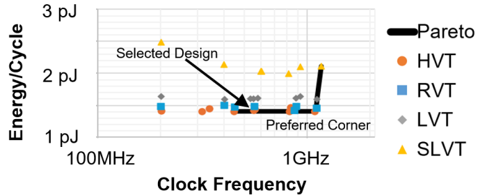
Fig. 4. Cortex-M0 average energy per cycle vs. clock frequency, shown for the matmul-int Embench workload. HVT, RVT, LVT, & SLVT for “High”, “Regular”, “Low” & “Super Low” V_T in the ASAP7 PDK [19].
