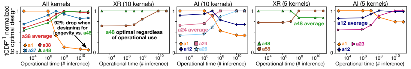
Fig. 9. Carbon efficiency (y-axis) normalized to the optimal design versus operational time (x-axis). To improve robustness against variations and uncertainty in estimating hardware usage, designers can trade-off tCDP optimality at a given operational time with another design that has a better average tCDP across a wide range of operational times.
